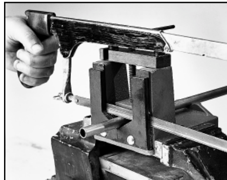
Fig. C4 — Parker's Tru-Kut sawing vise used with hacksaw
