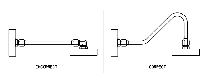
Fig. C13 — Use "S" bends to compensate for small variations in the tube length
