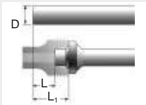
● Extra length
