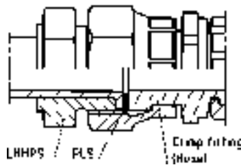
Tube to tube
