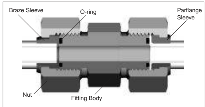
Fig. 1 – O-Lok Union cutaway with flanged and brazed assemblies
