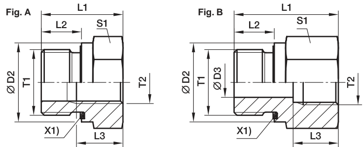
X1) Elastic-sealing ED
